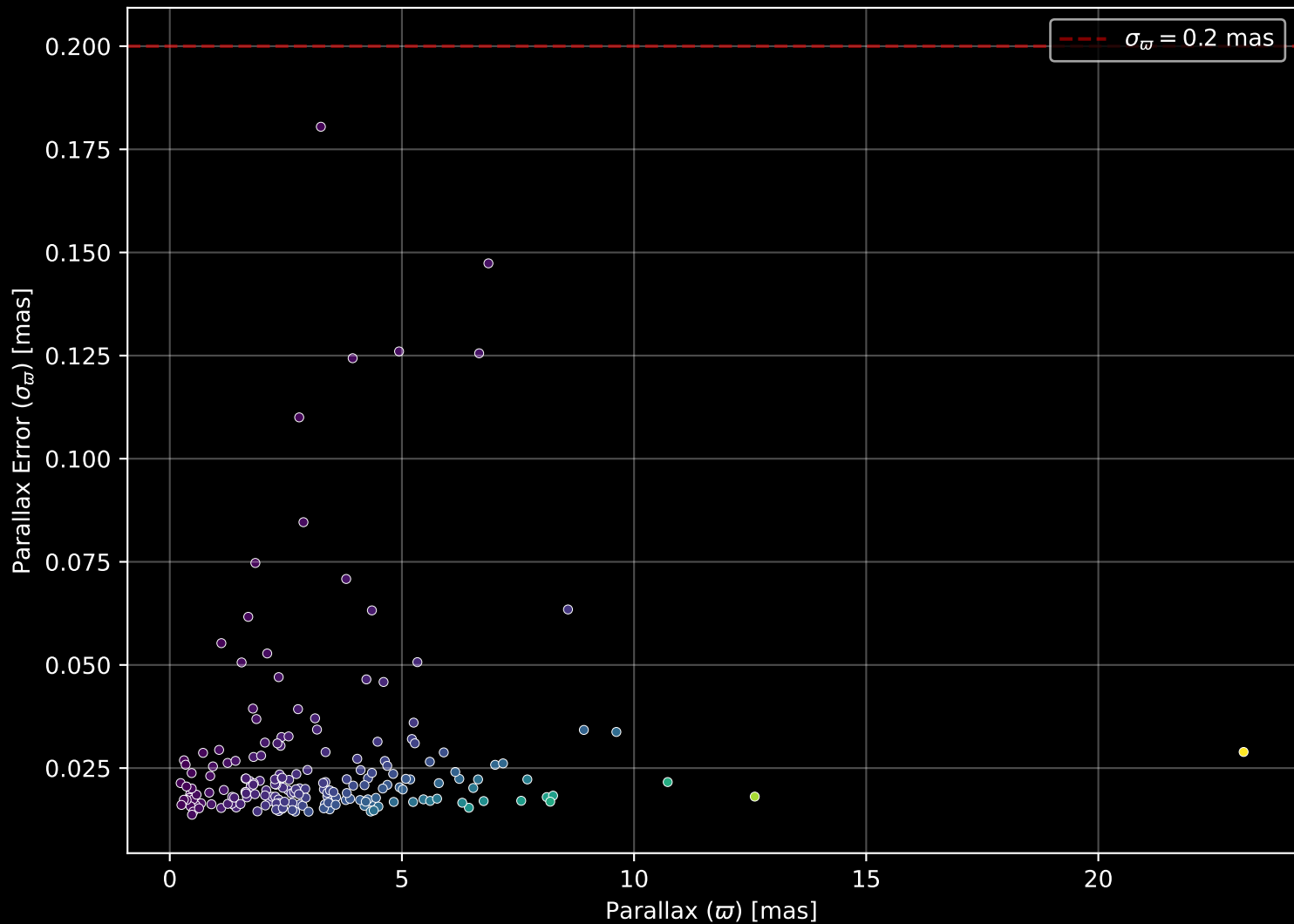
APOGEE DR17 Field: [K2_C3_055-47_btx] Parallax Quality (n= 198)
