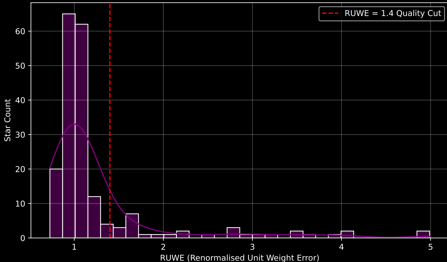
GAPOGEE DR17 Field [K2_C3_055-47_btx] RUWE Distribution (n= 193)
