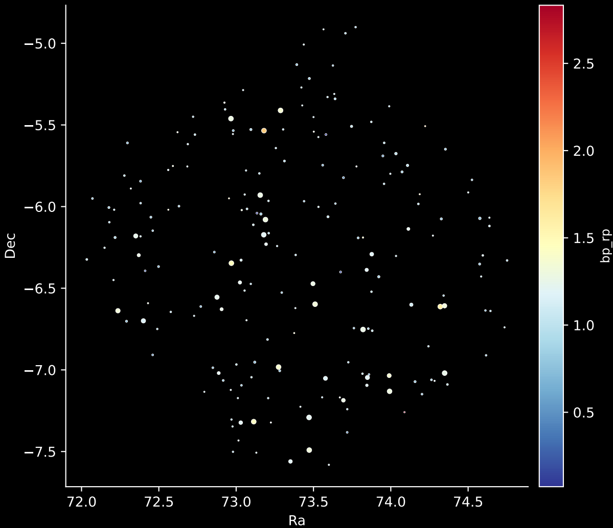
APOGEE DR17 Field: [K2_C3_055-47_btx] Stars: 198
