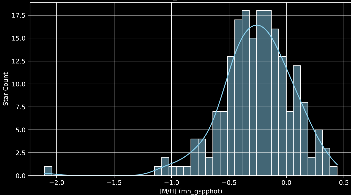
APOGEE DR17 Field: [K2_C3_055-47_btx [M/H] (mh_gspphot) (n= 197)
