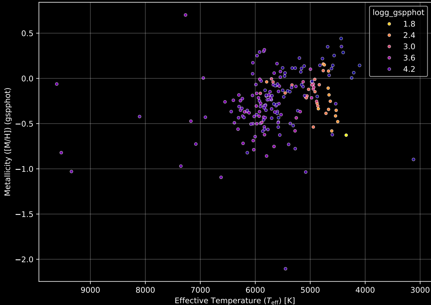
APOGEE DR17 Field: [K2_C3_055-47_btx] Stellar Population Parameters (n= 198)
