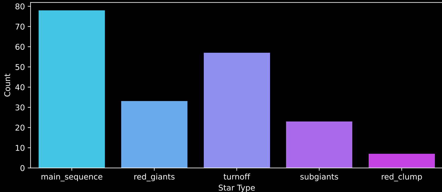
APOGEE DR17 Field: [K2_C3_055-47_btx] Count plot of Star Type
