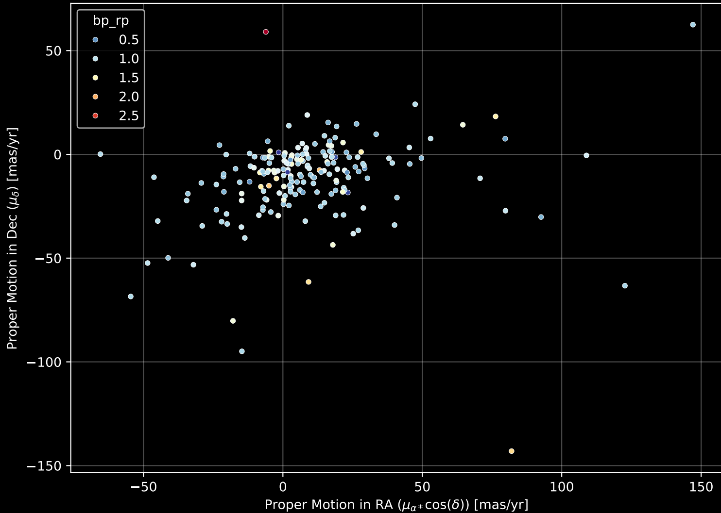
APOGEE DR17 Field: [K2_C3_055-47_btx] Proper Motion Diagram (n= 198)
